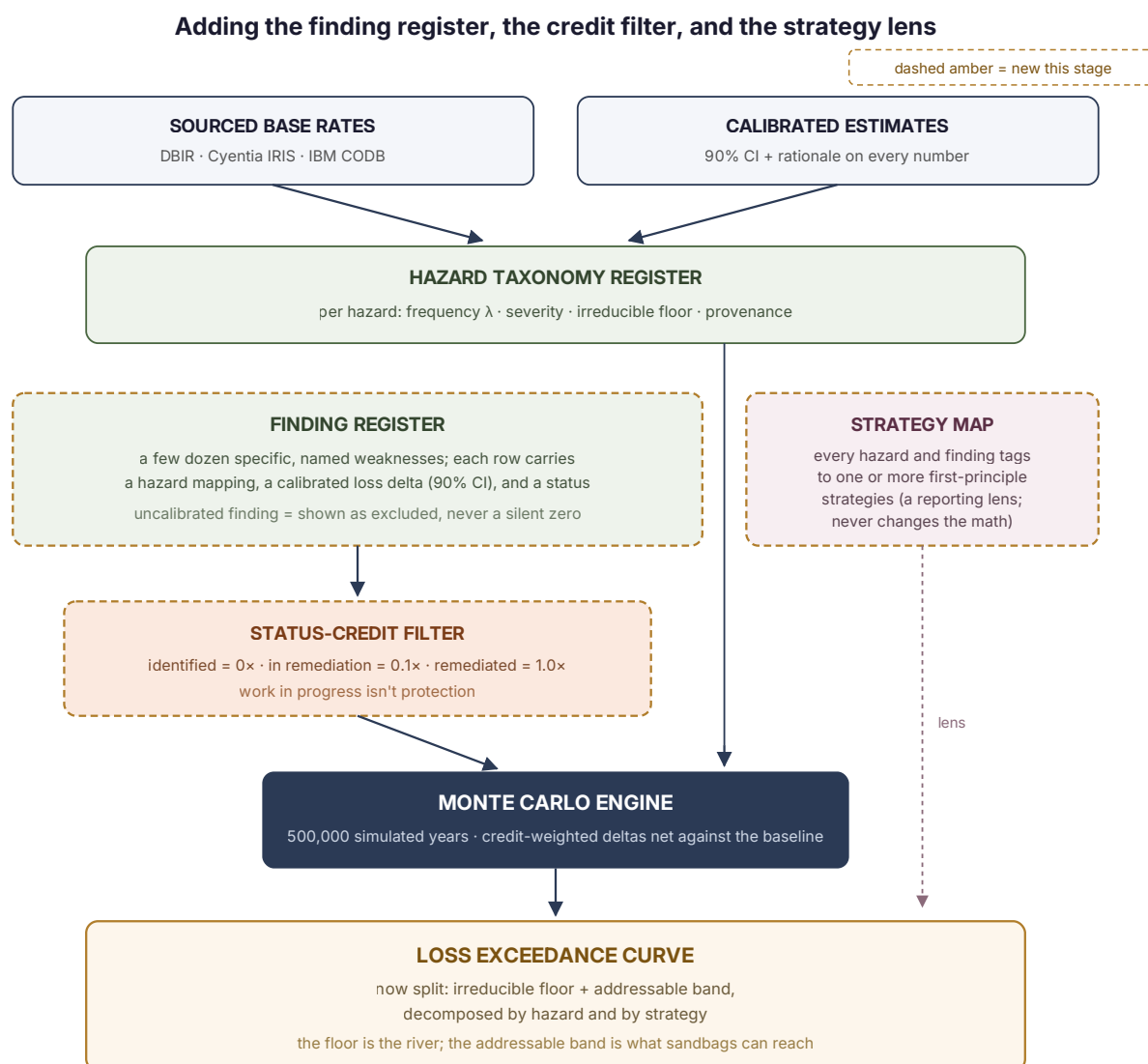
Figure 3. What changed: two new components between the hazard register and the engine. The finding register holds the company's specific, named weaknesses, each mapped to hazards, priced with a calibrated loss delta, and tracked by status; the status-credit filter converts status into earned credit (0x / 0.1x / 1.0x) before anything reaches the math. On the right, the strategy map tags every hazard and finding to one or more first-principle strategies; it's a reporting lens and never changes the curve. The output now shows the floor/addressable split.
