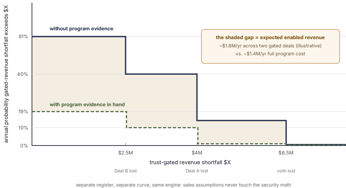
Figure 7. What you're looking at: the revenue-at-risk exceedance curve, built exactly like the loss curve but pointed at the pipeline: for every X, the annual probability that trust-gated revenue shortfall exceeds X. The upper solid line is Feynman without evidence in hand; the lower dashed line is with the program's evidence. The steps mark the individual deals. The shaded gap between the curves is the expected enabled revenue, about $1.8M a year here, and it's the number the program budget gets sized against from the growth direction. Illustrative figures, disguised like everything else.
