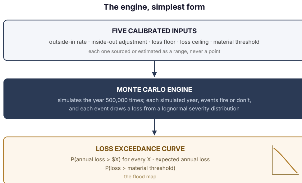
Figure 1. What you're looking at: the whole method at its simplest. Five calibrated inputs at the top, a Monte Carlo engine in the middle simulating the year half a million times, and the loss exceedance curve at the bottom. Every section that follows adds one layer to this diagram until the full production system stands at the end of the piece.
