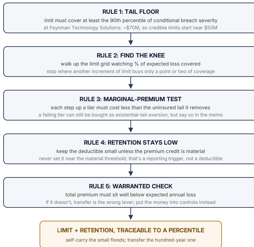
Figure 6. What you're looking at: the five rules as a decision flow, top to bottom, each with its test and its Feynman reading. The output at the bottom is the point: a limit and retention that trace to a percentile on the curve, defensible in front of a board or an underwriter, instead of a multiple of revenue somebody remembered from a webinar.
